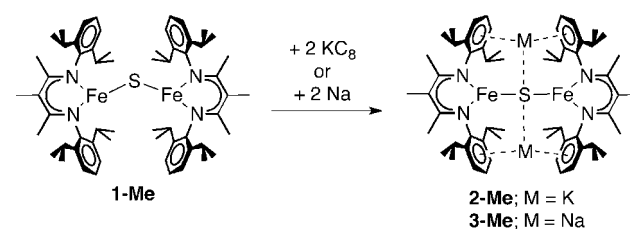
Scheme 2. Synthesis of the diiron(I) sulfide complexes.
