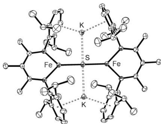
Figure 1. Thermal-ellipsoid plot of [\{K^{Me}L^{Me}Fe\}_2(\mu-S)] ( 2-Me ). Ellipsoids are set at 50% probability; hydrogen atoms omitted for clarity. The sodium analogue 3-Me has also been crystallographically characterized, and is shown in the Supporting Information.
